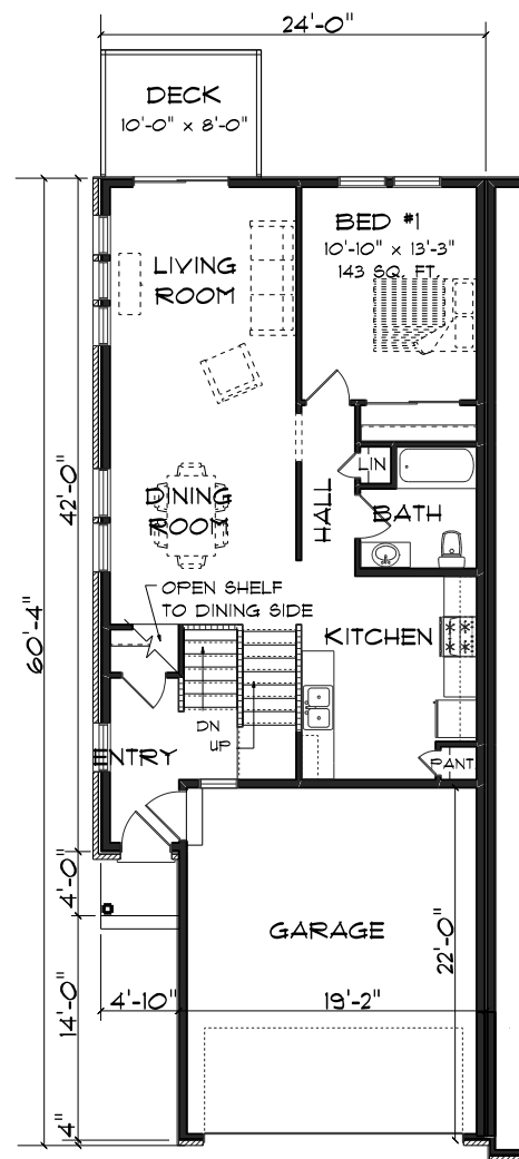
UPPER LEVEL PLAN
