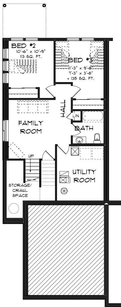
LOWER LEVEL PLAN
